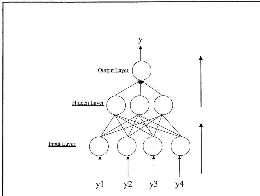
Figure 1 Feed-Forward Neural Network.
