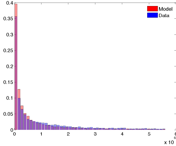
Figure 4: Distribution of foreign sales: model vs. data.
