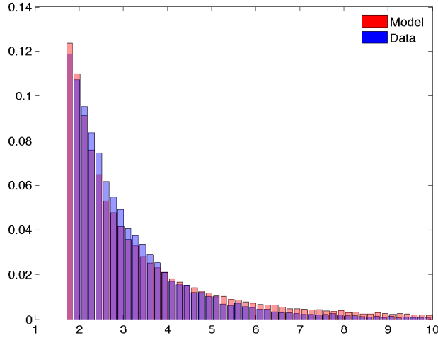
Figure 5: Distribution of markups: model vs. data.
