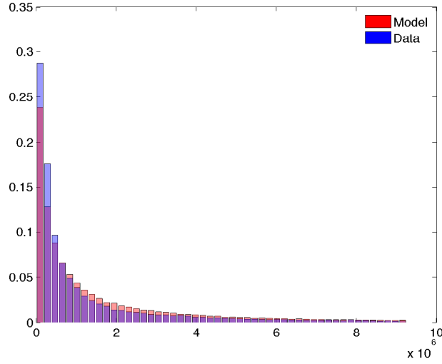
Figure 3: Distribution of domestic sales: model vs. data.
