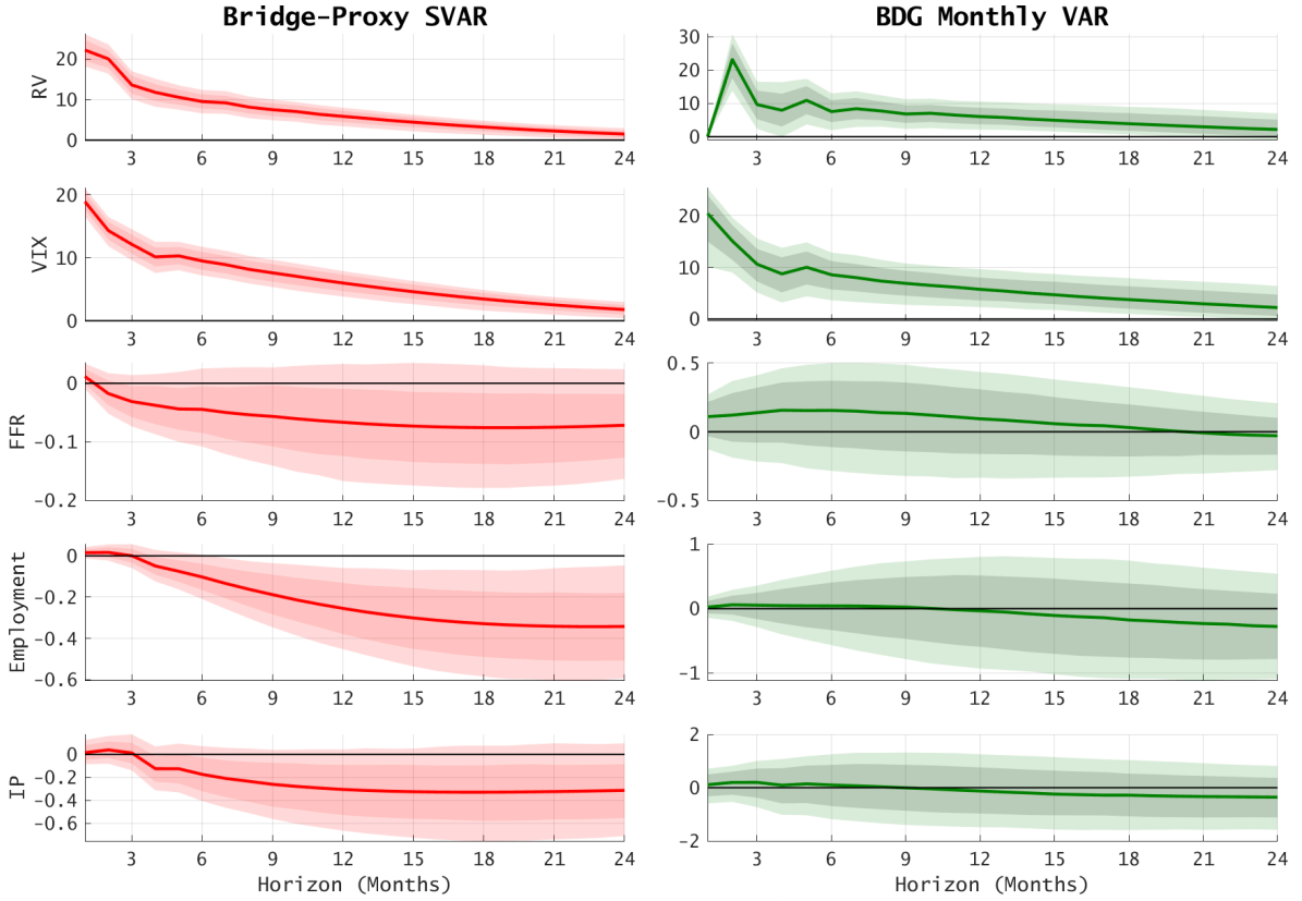
Figure 3: Comparison with BDG
