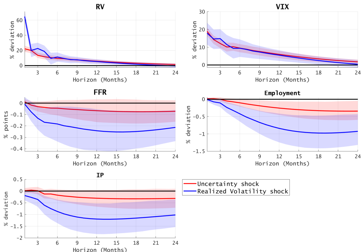
Figure 4: Comparison of IRFs: Uncertainty versus Realized Volatility Shocks
