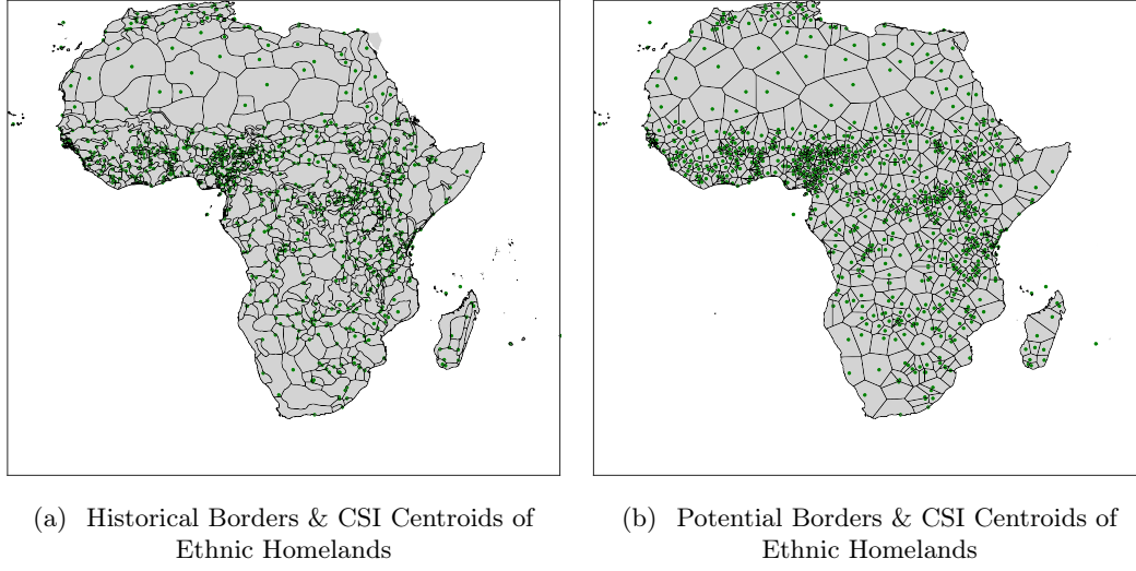
Figure C.2: Historical Ethnic Borders, CSI Centroids and CSI Potential (Voronoi) Borders in Africa
