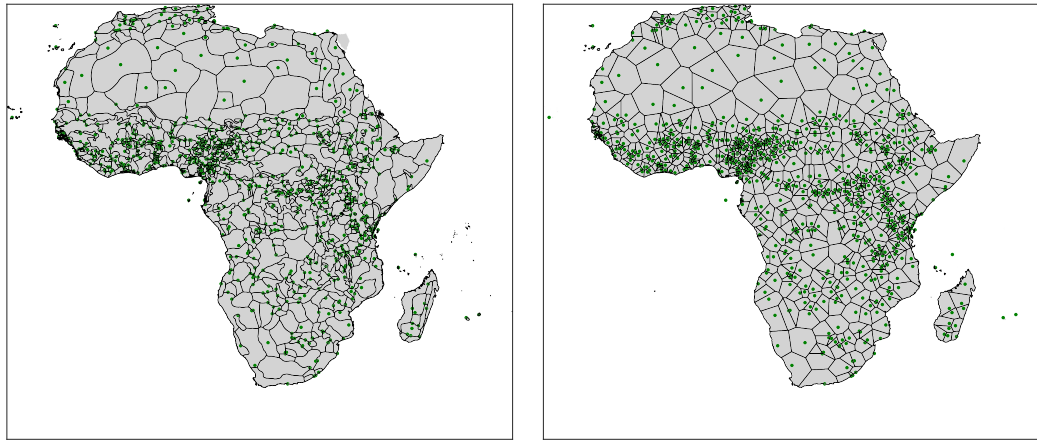
(a) Historical Borders & CSIMEAN Centroids of Ethnic Homelands (b) Potential Borders & CSIMEAN Centroids of Ethnic Homelands
