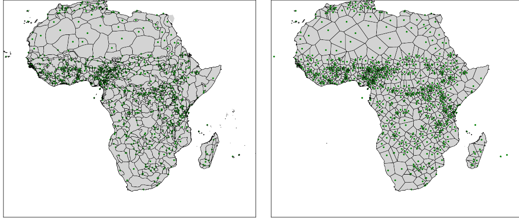
(a) Historical Borders & EA Centroids of Ethnic Homelands
